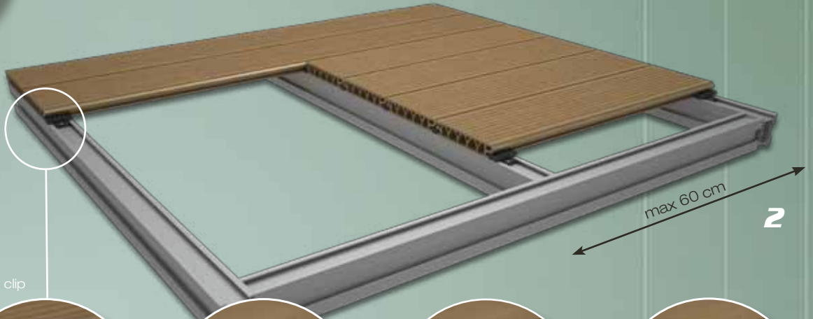
Assembly with joiner
